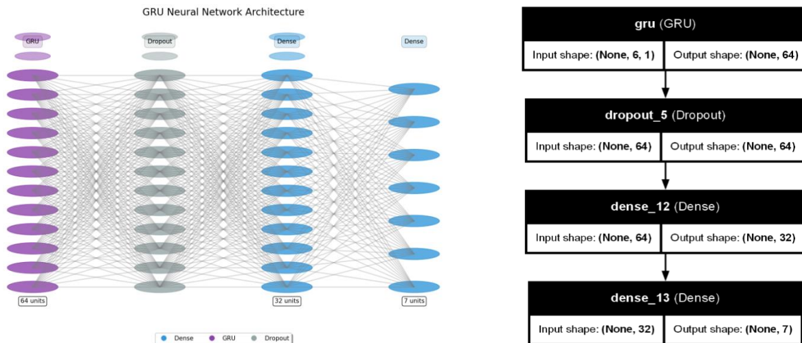
Figure 59 : architecture de GRU training
