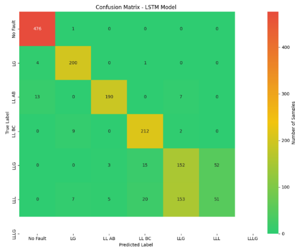
Figure 65 : Matrice de confusion LSTM
