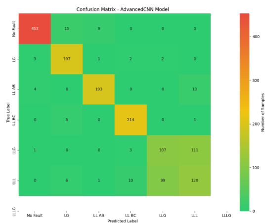
Figure 45 : Matrice de confusion AdvancedCNN
