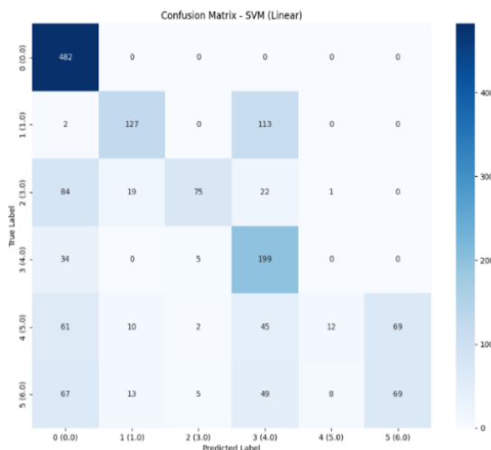
Figure 20 : Confusion de matrice SVM SVM Linear
