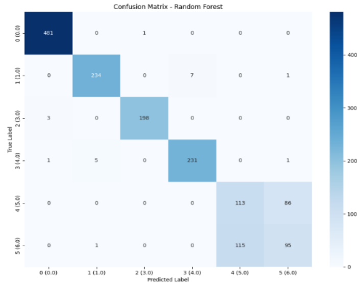
Figure 26 : Confusion de matrice Random Forest
