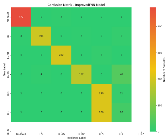
Figure 60 : Matrice de confusion Improved FNN
