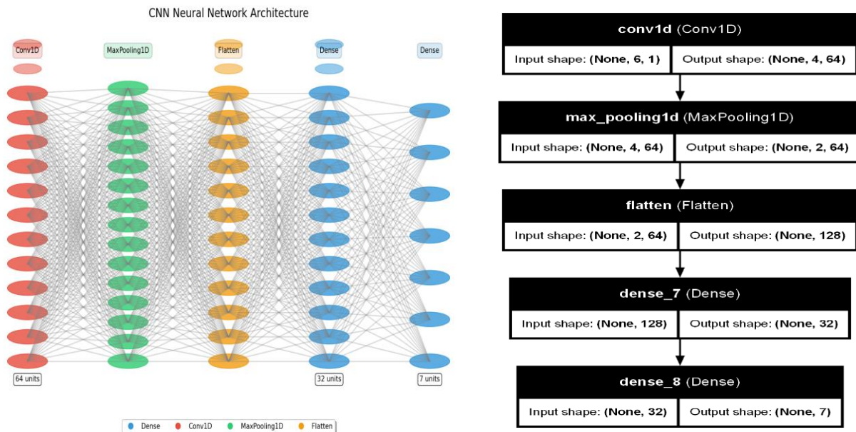
Figure 40 : architecture de CNN training
