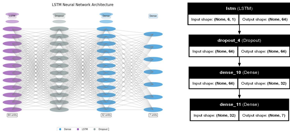
Figure 69 :Architecture de LSTM training
