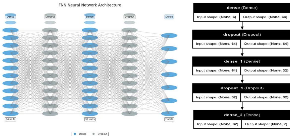
Figure 64 : architecture de Improved FNN training
