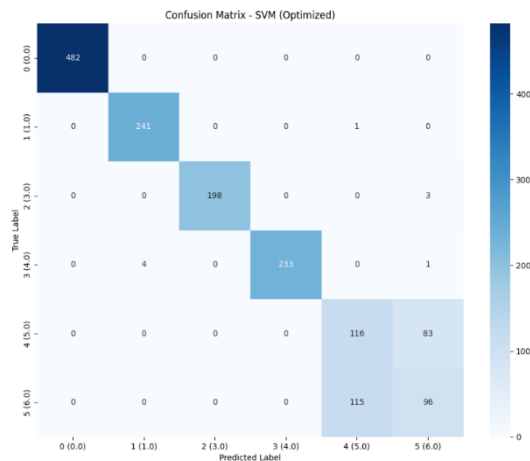
Figure 24 : Matrice de confusion SVM Optimized
