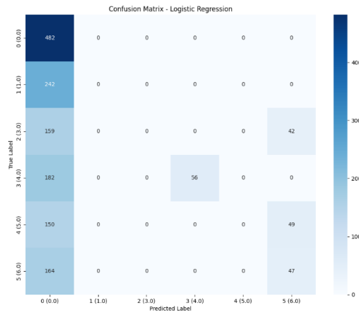
Figure 31 : Confusion de matrice logistic Regression
